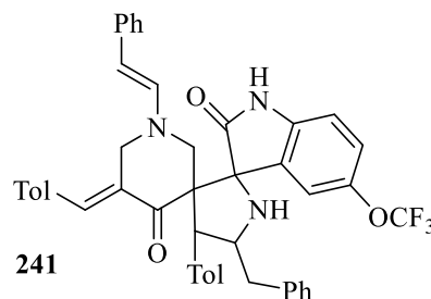
Figure 22. Chemical structure of phtalazine derivatives 234-241
